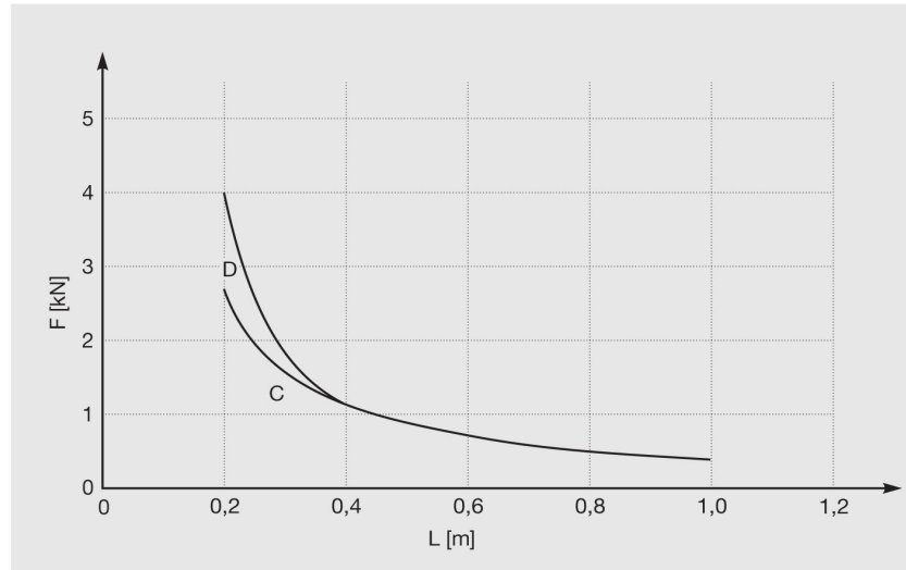
Endefeste WBD 41-75/65/3,0 D. Belastningsdiagram
