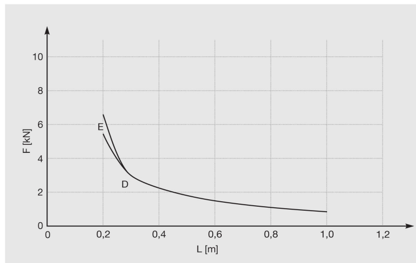
Endefeste WBD 41-75/65/3,0 D. Belastningsdiagram
