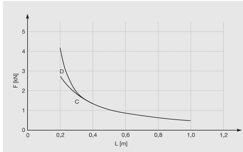
Endefeste WBD 41-75/75/3,0 D. Belastningsdiagram
