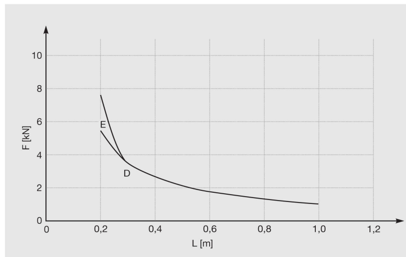
Endefeste WBD 41-75/75/3,0 D. Belastningsdiagram
